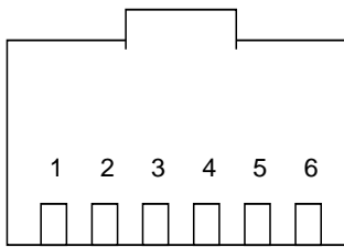
Figure 8. RJ11 “Customer” 1-Wire Interface
