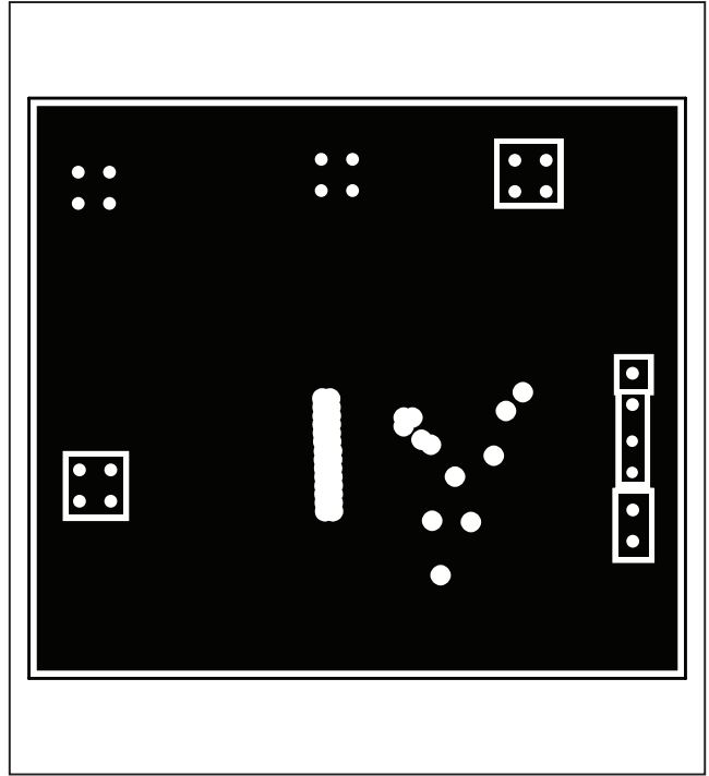
Figure 4. MAX15066 EV Kit PCB Layout—Inner Layer 2
