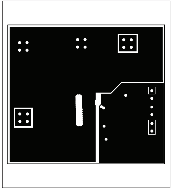
Figure 5. MAX15066 EV Kit PCB Layout—Inner Layer 3
