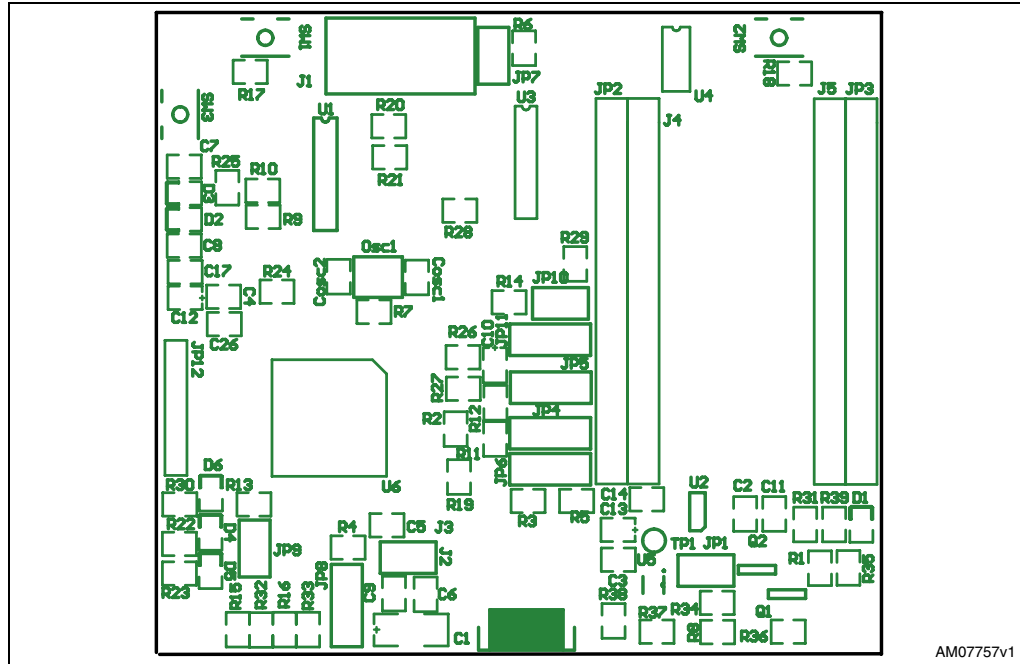
Figure 2. Top silk screen of the eMotion kit
