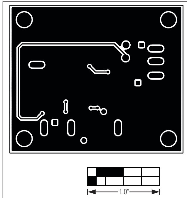
Figure 4. MAX9934T EV Kit PCB Layout—Solder Side
