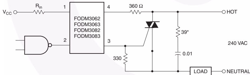
Figure 10. Hot-Line Switching Application Circuit
