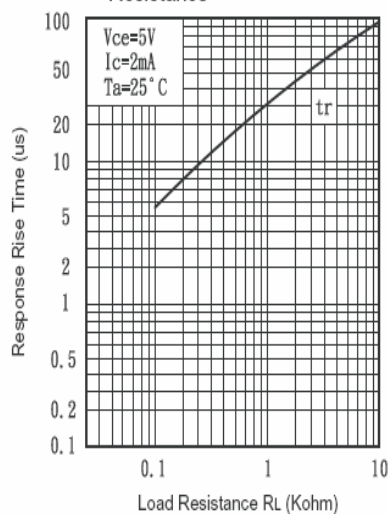
Fig.10 Response Time vs. Load Resistance
