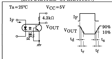
SWITCHING CHARACTERISTICS - R_{BE} (SATURATED OPERATION)
