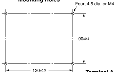
Mounting Holes
