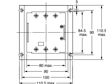
Note: With terminal cover.
