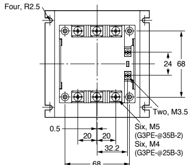
Note: Without terminal cover.
