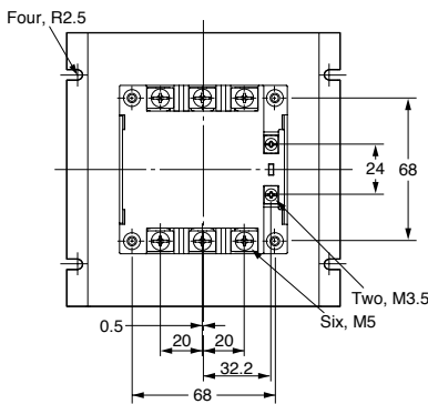
Note: Without terminal cover.
