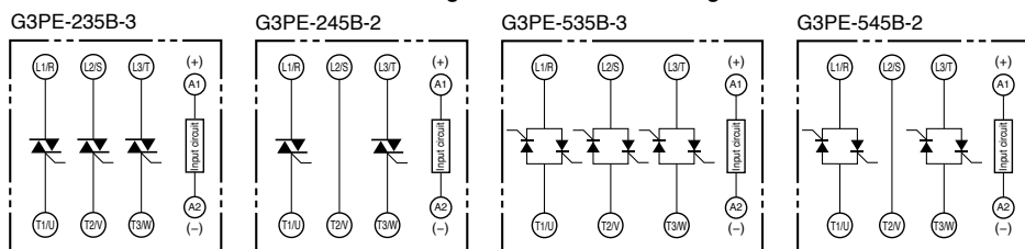
Terminal Arrangement/Internal Circuit Diagram
