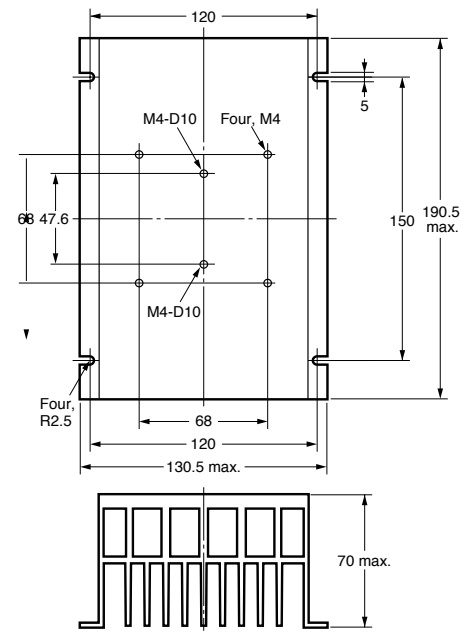
Mounting Holes
