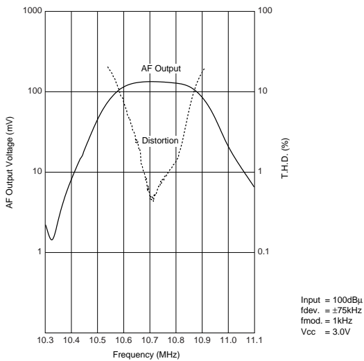
CDSCB10M7GA105A-R0
