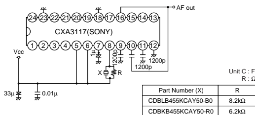
CXA3117
