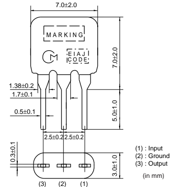
SFELF10M7HA00-B0
