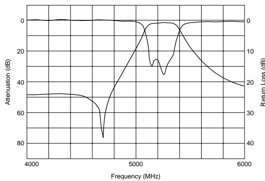
Pass Band: DFCEB35G25LAHAA
