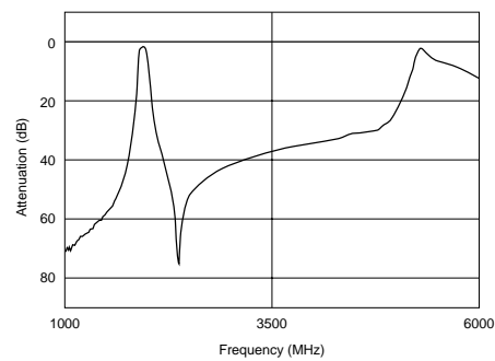
Spurious: DFCH31G95HDHAA
