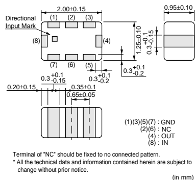
LFL21_TC Series
