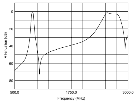
Spurious: DFCH3897MHDJAA
