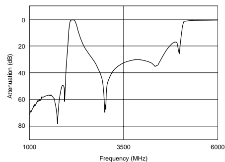
Spurious: DFCH32G14HDHA
