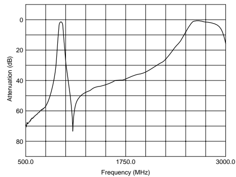
Spurious: DFCH3942MHDJAA
