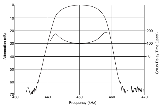
IFT+CFWLA450KF1Y-B0
