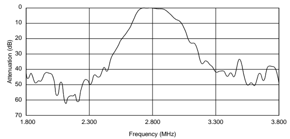
SFSKB2M80GF00-R1
