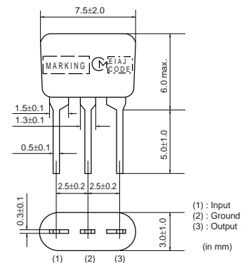
SFELG10M7FA00-B0
