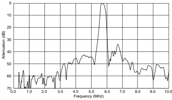
SFSRA5M74CF00-B0
