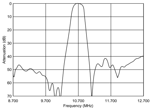
SFELG10M7FA00-B0
