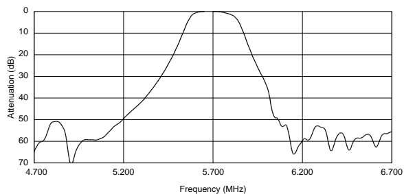
SFSKB5M70GF00-R1
