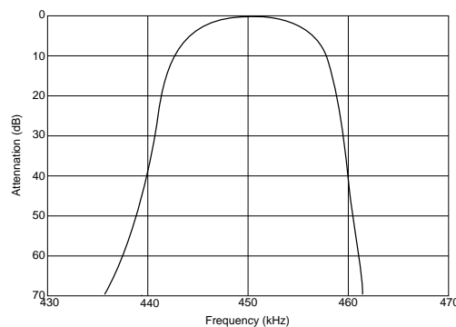
IFT+CFWLA450KFFA-B0
