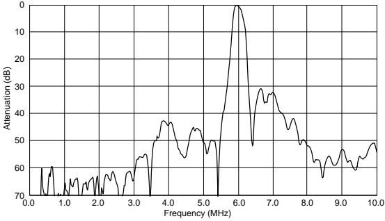
SFSRA6M00CF00-B0
