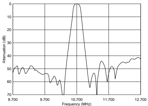
SFELG10M7HA00-B0
