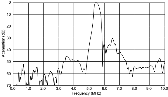
SFSRA5M50DF00-B0
