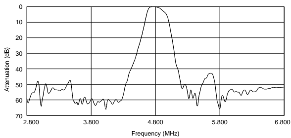
SFSKB4M80GF00-R1
