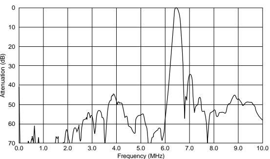
SFSRA6M50BF00-B0
