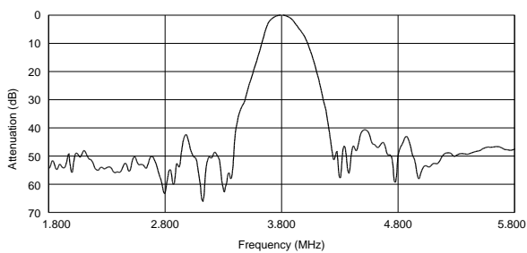
SFSKB3M80GF00-R1
