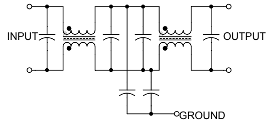
Figure 4. Internal Schematic
