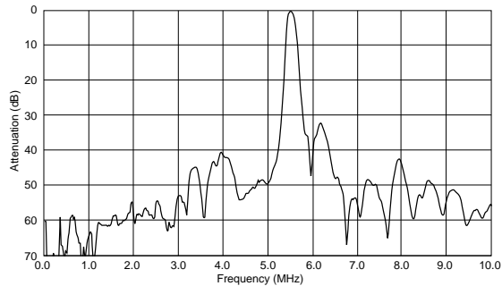
SFSRA5M50BF00-B0
