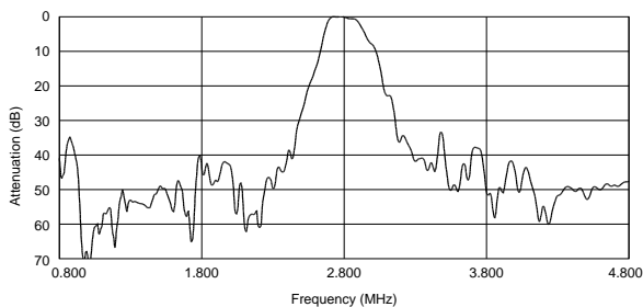
SFSKB2M80GF00-R1
