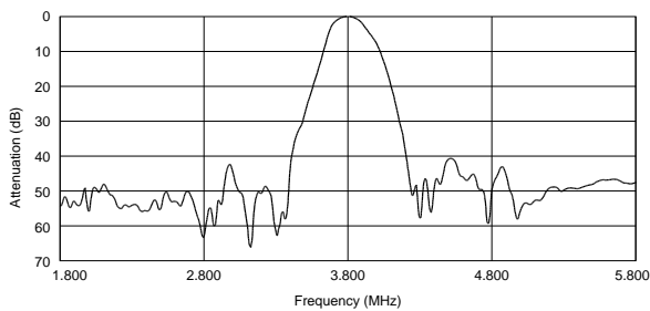
SFSKB3M80GF00-R1
