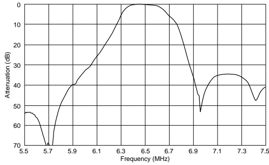
SFSRA6M50DF00-B0
