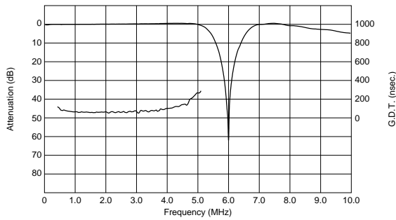
TPSKA6M00B00-R1
