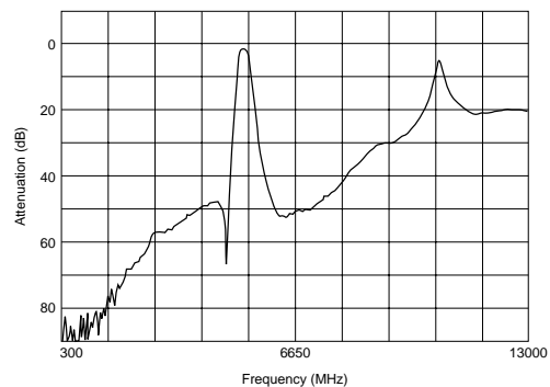
Spurious: DFCEB35G25LAHAA
