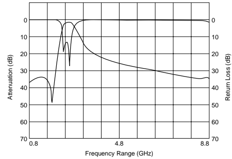
Frequency Characteristics
