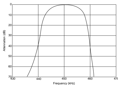
IFT+CFWLA450KFFA-B0
