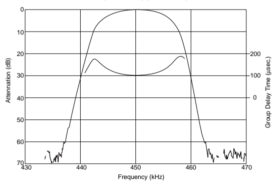
IFT+CFWLA450KF1Y-B0
