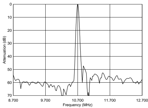
SFVLF10M7MF00-B0
