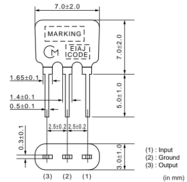
SFVLF10M7MF00-B0
