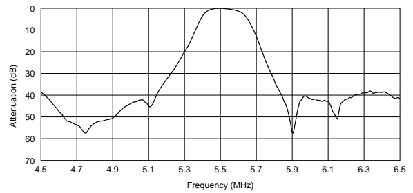
SFSKA5M50CF00-R1
