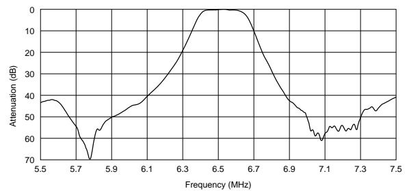
SFSKA6M50CF00-R1
