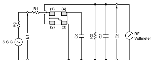
SFSKB2M80GF00-R1/SFSKB3M20FF00-R1
