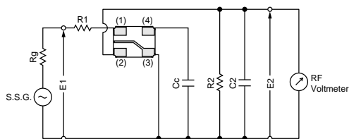
SFSKB4M80GF00-R1
