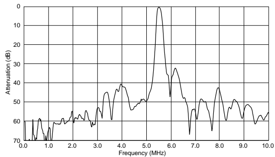
SFSRA5M50BF00-B0
