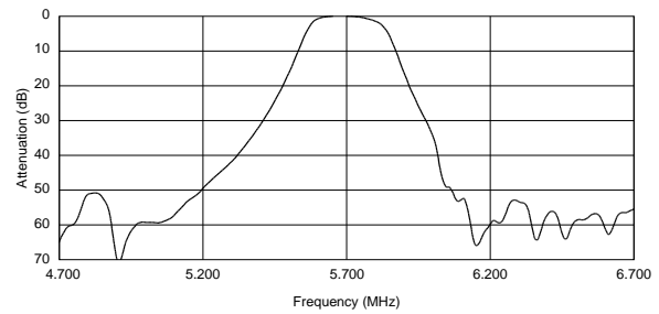
SFSKB5M70GF00-R1
