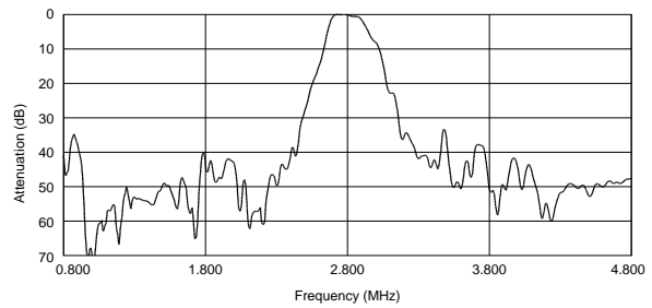
SFSKB2M80GF00-R1
