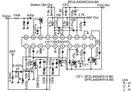
SFPLA450KH1A-B0/BFULA450KC004-B0
