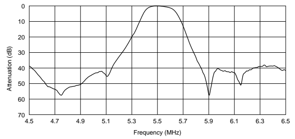
SFSKA5M50CF00-R1
