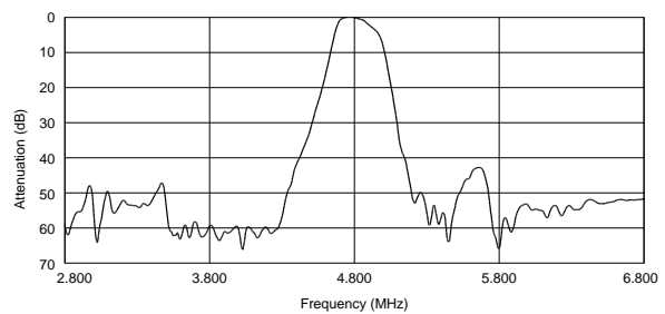
SFSKB4M80GF00-R1
