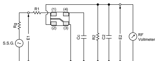
SFSKB2M30GF00-R1/SFSKB3M20GF00-R1
