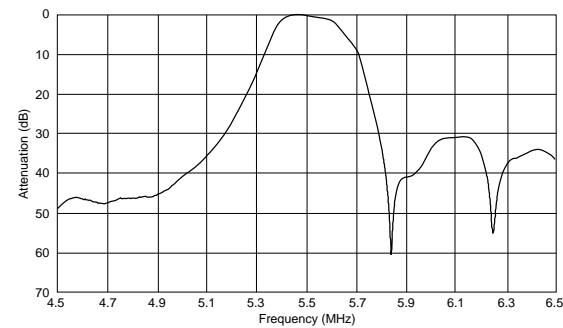
SFSRA5M50CF00-B0
