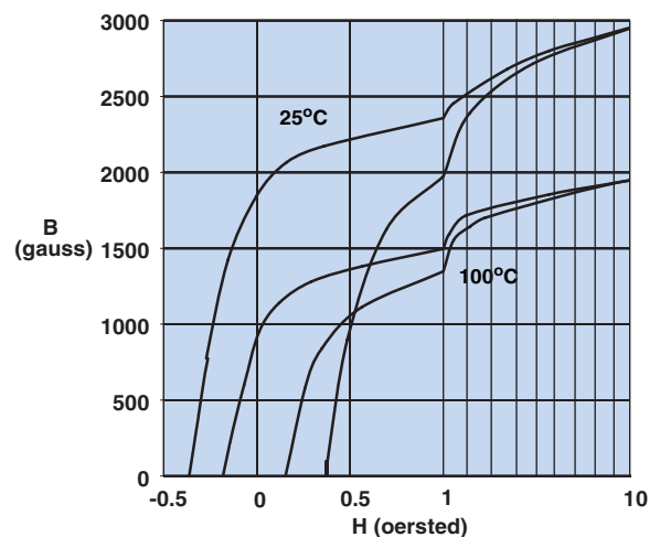
Hysteresis Loop
