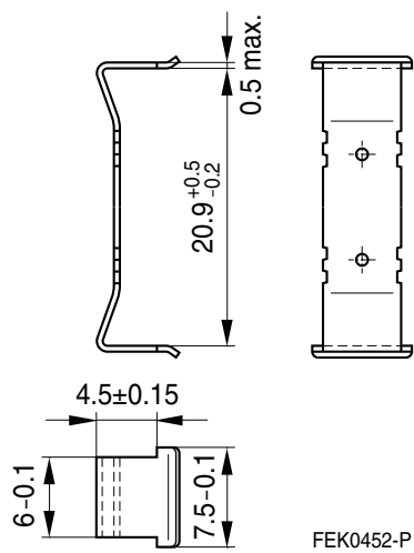
Figure 3, Yoke
