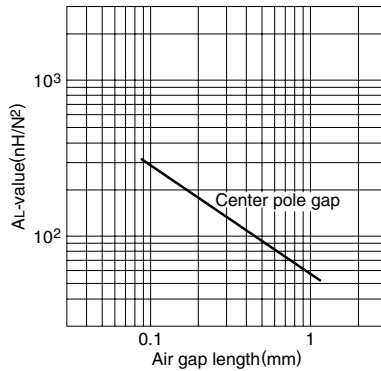
AL-value vs. Air gap length for PC44LP23/8 core (Typical)
