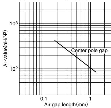
AL-value vs. Air gap length for PC44LP22/13 core (Typical)
