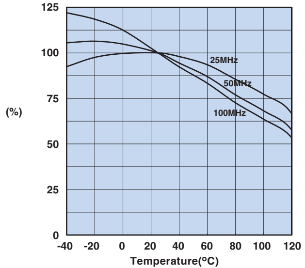
Figure 14 Percent of Original Impedance vs. Temperature Measured on a 2643000301 using the HP4291A.
