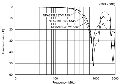
NFA21SL_V_45 Series
