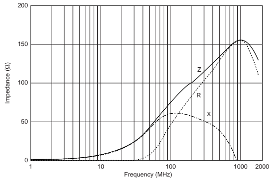
BLA2ABD750SN4
