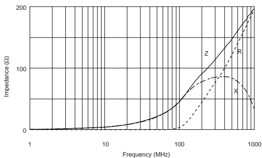
BLA2ABB470SN4
