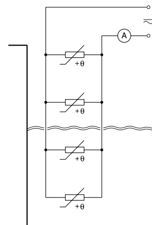
The PTC thermistors located above the fluid level will be heated to a temperature greater than T_n . When immersed they are cooled such that their resistance value is reduced.
