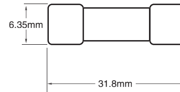
Dimensions mm/(inches)
