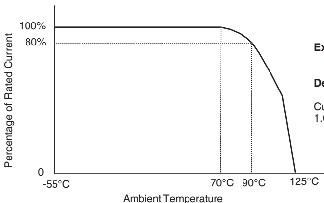
Current vs. Temperature Derating Guide
