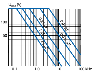
MMK7.5 ... 37.5 400/200
