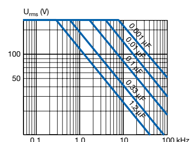
MMK7.5 ... 37.5 1000/250
