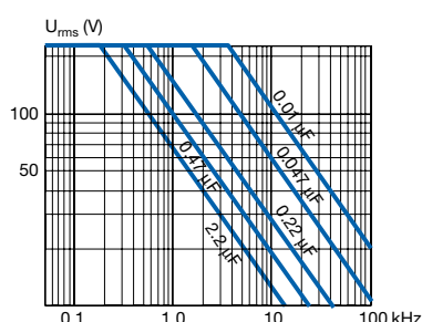
MMK7.5 ... 37.5 630/220
