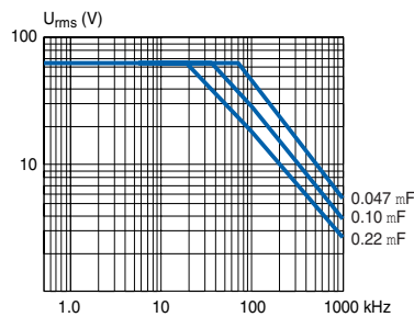
SMR5 100/63
