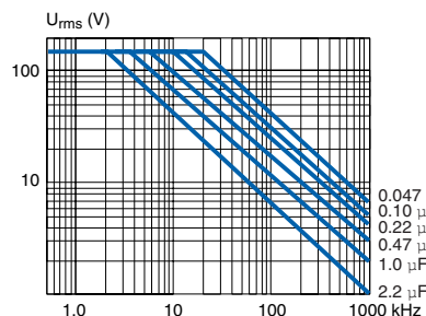
SMR7.5 ... 27.5 250/160
