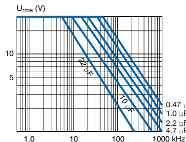
SMR7.5 ... 27.5 50/30
