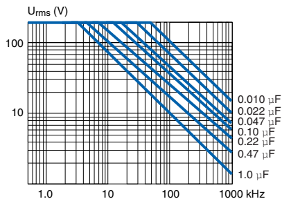
SMR7.5 ... 27.5 400/200
