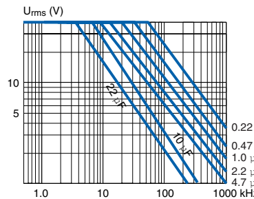
SMR7.5 ... 27.5 63/40
