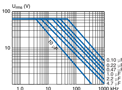
SMR7.5 ... 27.5 100/63
