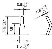
(Terminal dimensions)
