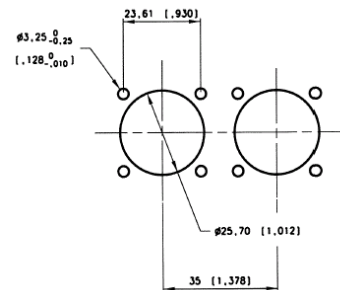
Panel Drilling
