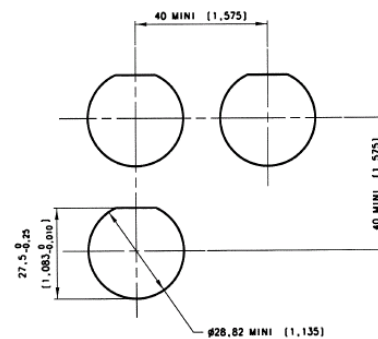
Panel Drilling
