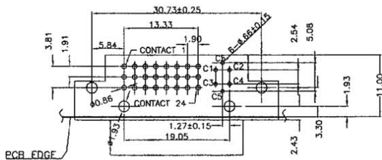
RECOMMENDED P.C.B LAYOUT TOLERANCES: ±0.05mm
