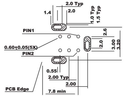
Recommended PCB Footprint
