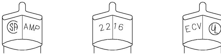
STAMPING DETAIL
