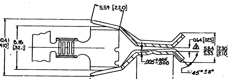
SECT. A-A
