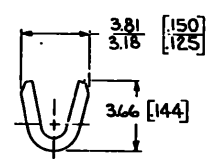
SECT. C-C
