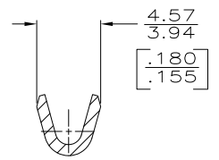
SECTION A-A SCALE 5:1
