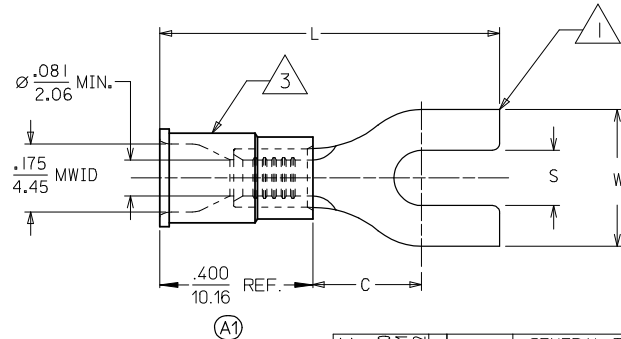
CUSTOMER DRAWING
