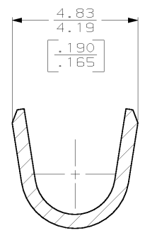
SECTION B-B SCALE 10:1
