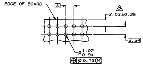
RECOMMENDED MOUNTING PATTERN
