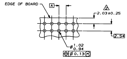
RECOMMENDED MOUNTING PATTERN
