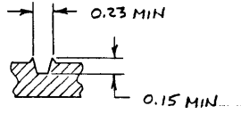
SECTION A-A TYP. SERRATION
