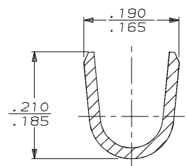
SECTION B-B SCALE 8:1
