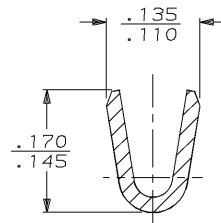
SECTION A-A SCALE 8:1
