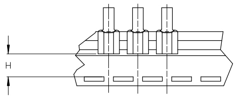
TAPE MOUNTING DETAIL
