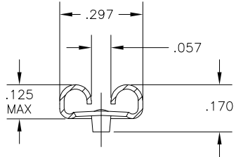
SECTION Y-Y
