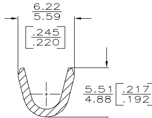
SECTION Y-Y
