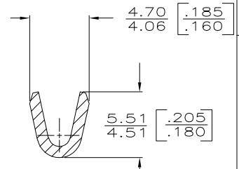
SECTION X-X
