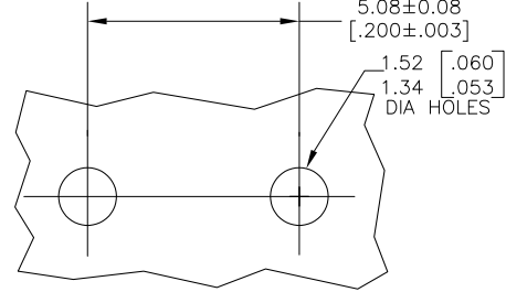
P.C. BOARD HOLES SCALE 10:1
