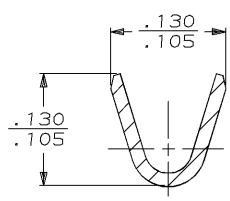
SECTION B-B SCALE 10:1
