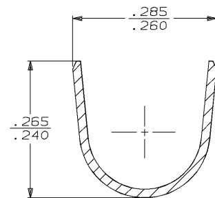
SECTION B-B SCALE 8:1
