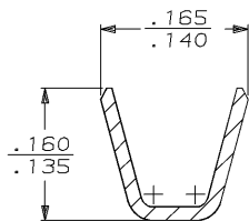
SECTION A-A SCALE 8:1
